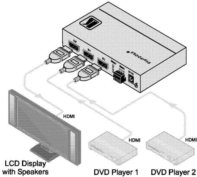
Figure 2: VS-211H Automatic HDMI Standby Switcher Connections
