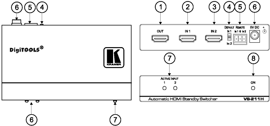
Figure 1: VS-211H Automatic HDMI Standby Switcher
