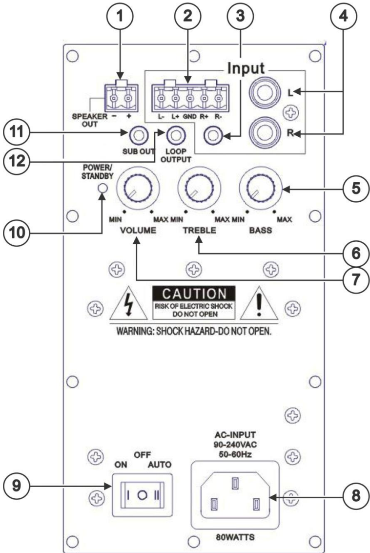
Figure 3: Tavor 5-O Active Speaker
