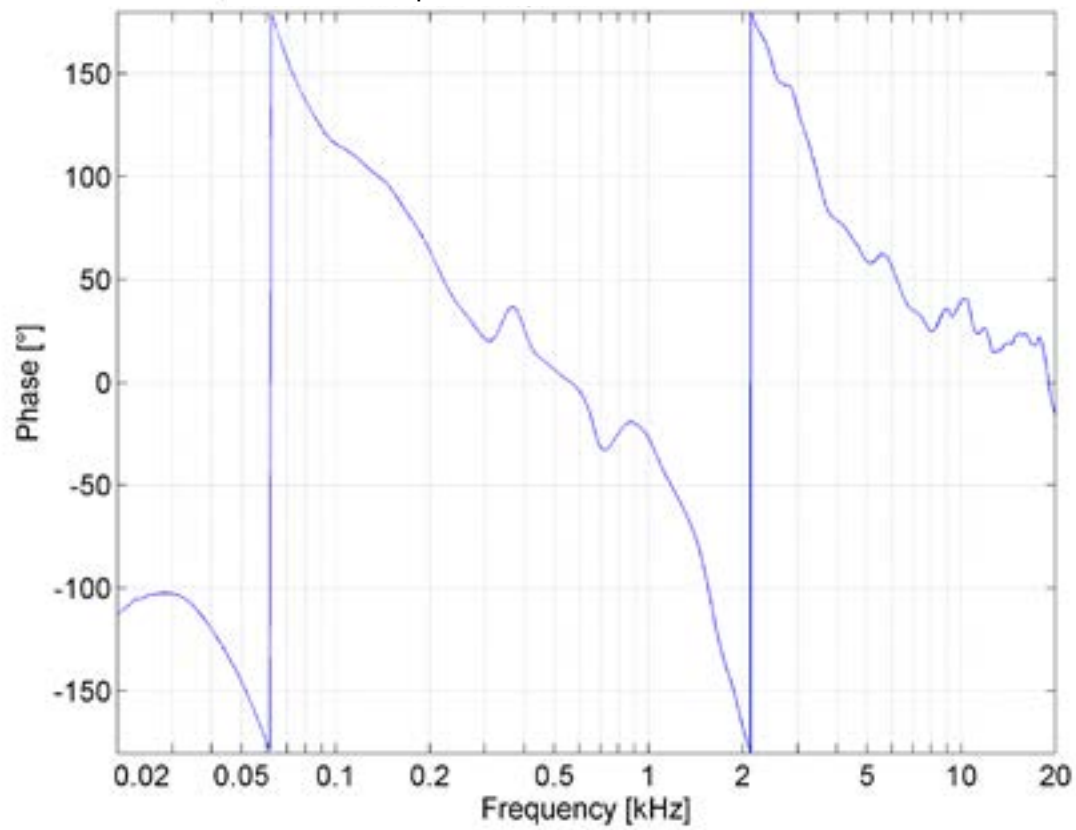
BT-8 Phase response
