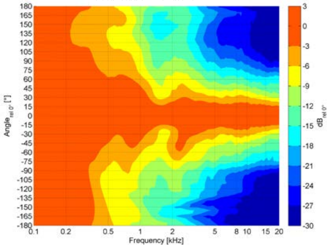
Vertical isobars: BT-8 Passive
