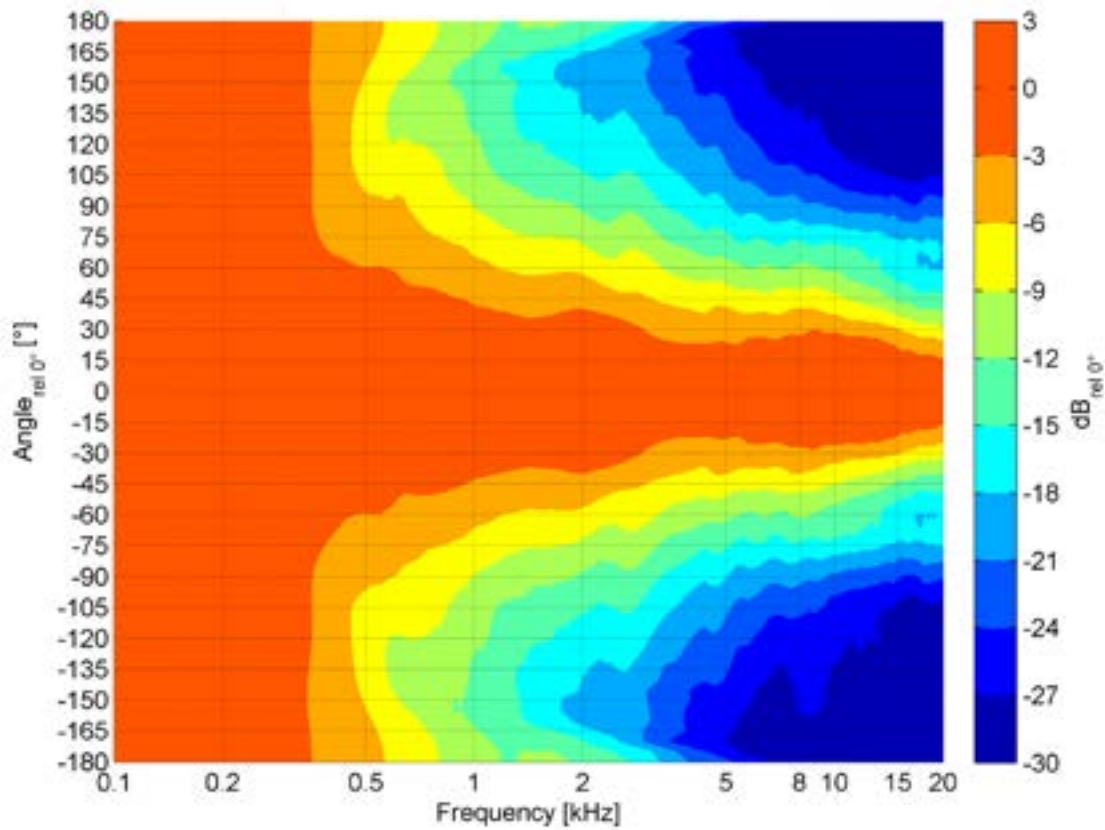
Horizontal isobars: BT-8 Passive
