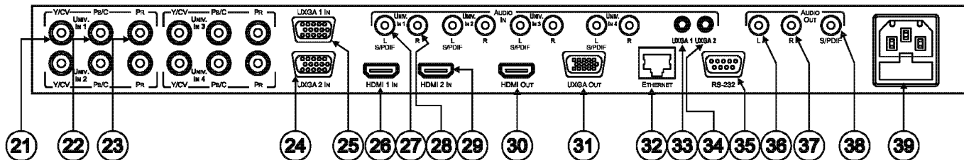
Figure 2: VP-729 Presentation Switcher / Scaler Rear Panel
