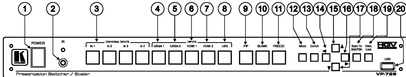
Figure 1: VP-729 Presentation Switcher / Scaler Front Panel
