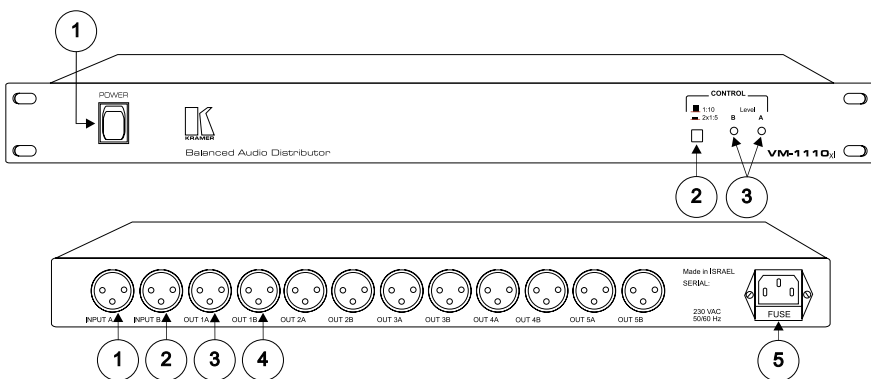
Figure 1: VM 1110xl Balanced Audio Distributor
