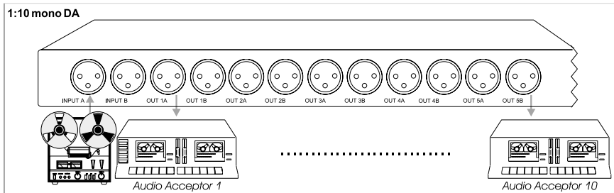
Figure 2: Mono (1:10) DA Configuration
