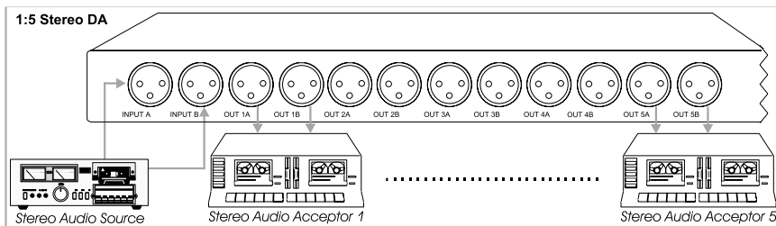
Figure 3: Stereo (1:5) DA Configuration
