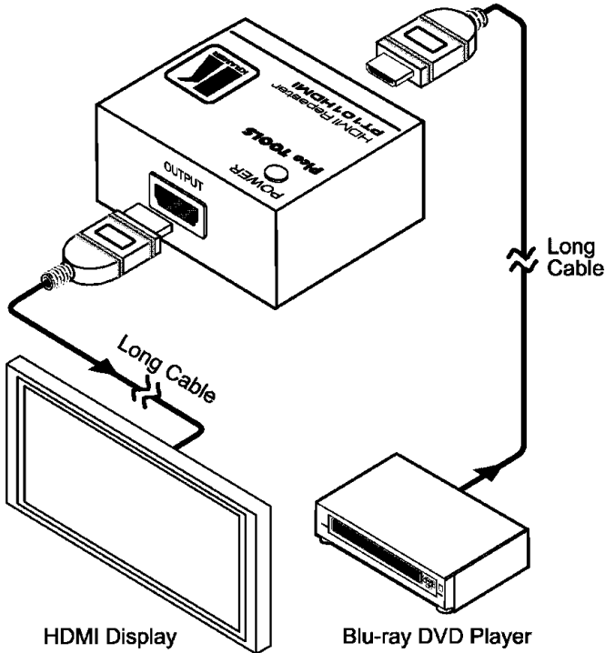
Figure 2: Connecting the PT-101HDMI HDMI Repeater
